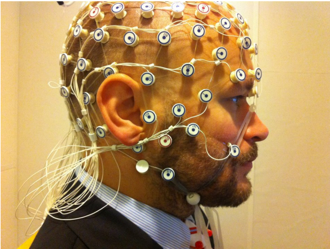
Figure 1.16 EEG recording
