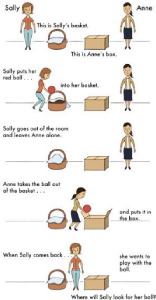
Figure 4.15: False-belief test.
